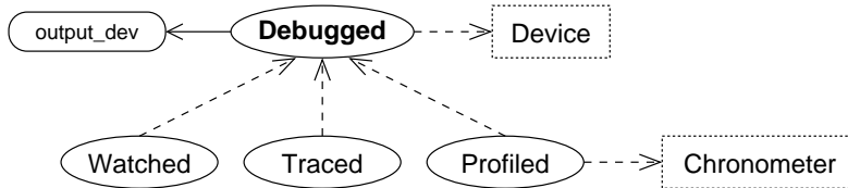
Figure 4.32: EPOS family of debugging and profiling aspects.
