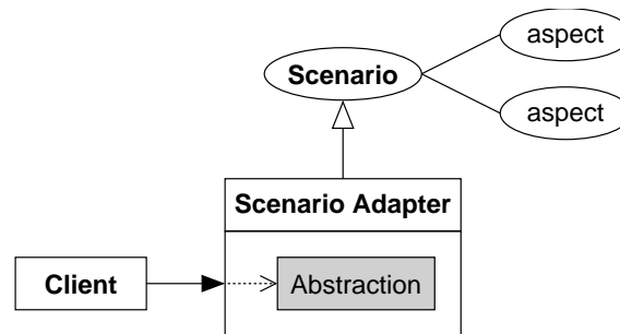
Figure 3.9: The general structure of a scenario adapter.
