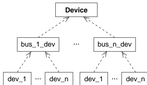
Figure 4.20: EPOS family of device abstractions.
