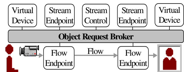
Figure 1. The CORBA streaming mechanism
