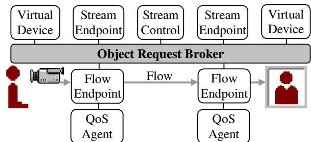
Figure 4. The Quartz/CORBA framework
