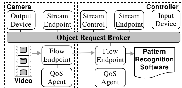
Figure 6. Software model of the pattern recognition mechanism
