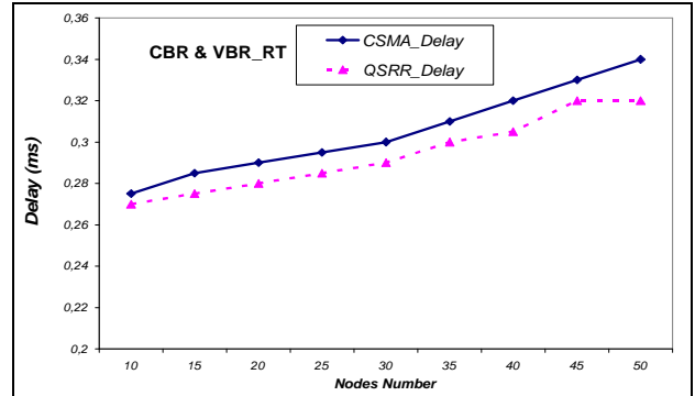
Figure 2. Delay evolution for applications 50% CBR & 50% VBR_RT
