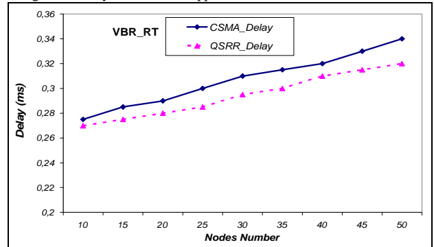
Figure 3. Delay evolution for applications 0% CBR & 100% VBR_RT
