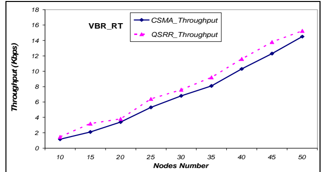
Figure 6. Throughput evolution for applications 0%CBR&100%VBR_RT
