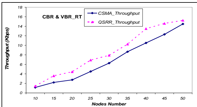
Figure 5. Throughput evolution for applications 50%CBR&50%VBR_RT
