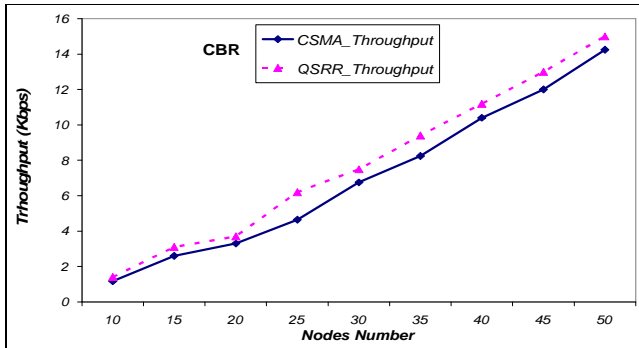
Figure 4. Throughput evolution for applications 100%CBR&0%VBR_RT
