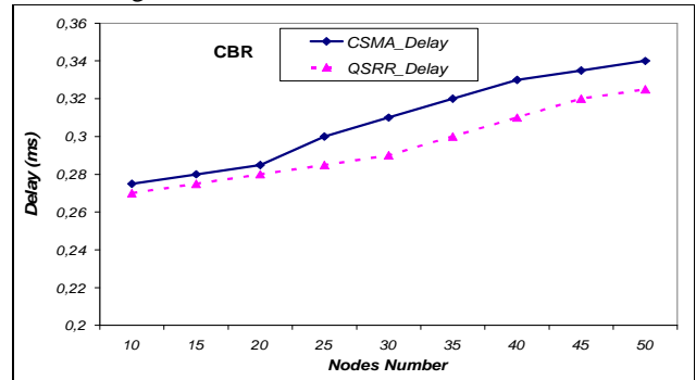
Figure 1. Delay evolution for applications 100% CBR & 0% VBR_RT
