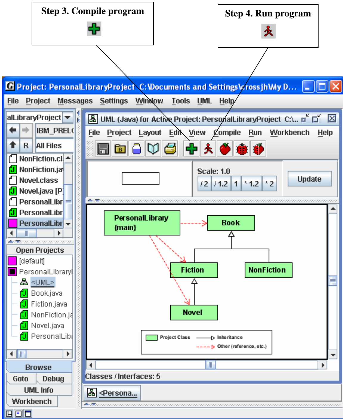
Figure 3-6. After loading file into CSD Window
