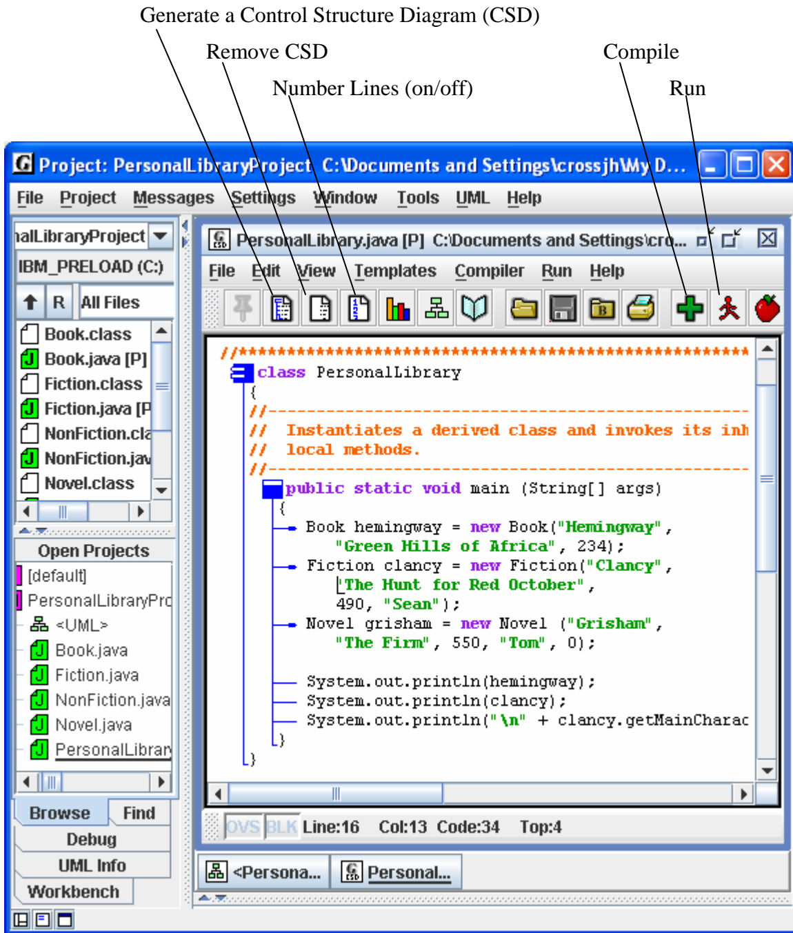
Figure 3-5. After the CSD is generated
