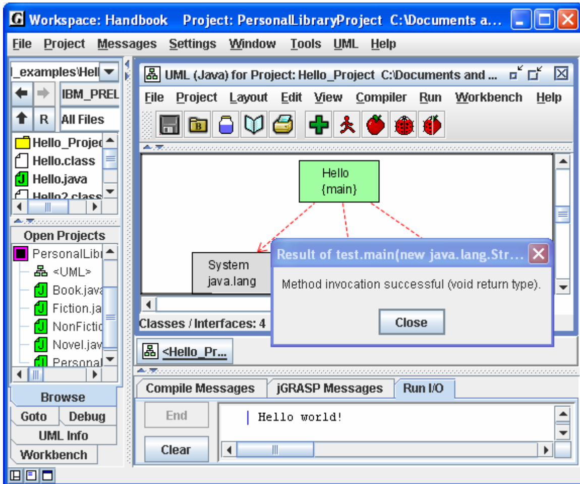
Figure 6-3. Invoking a static method from a class
