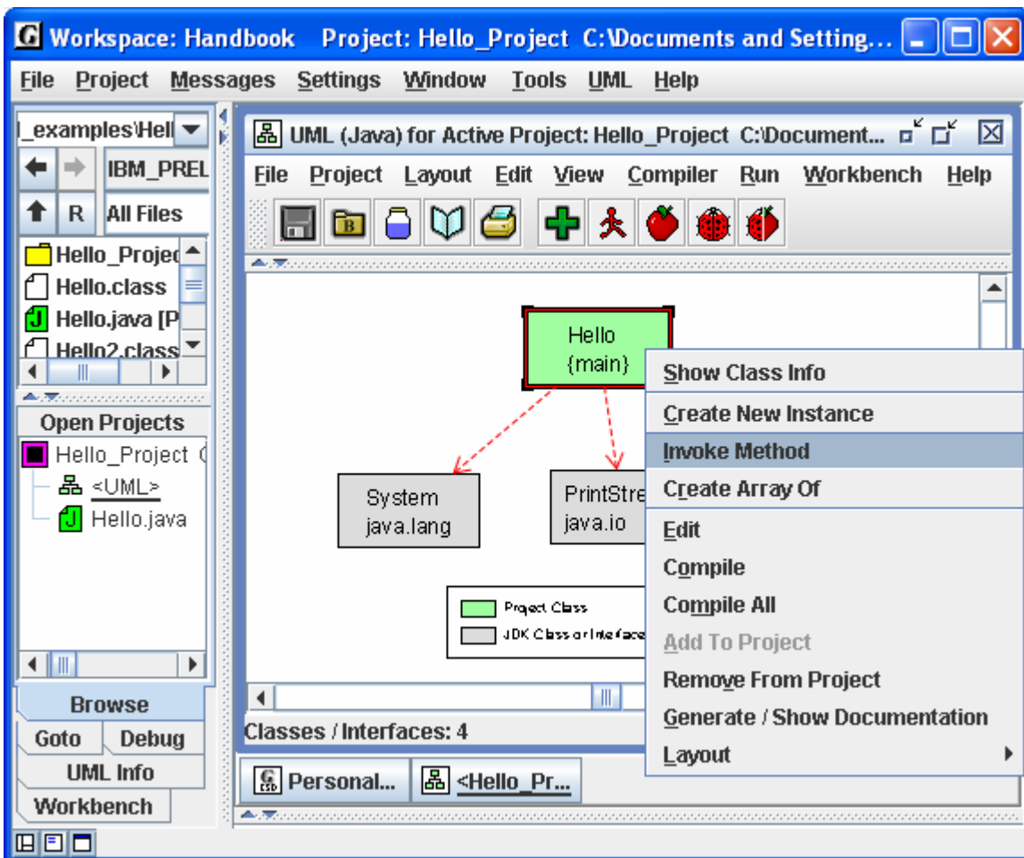
Figure 6-1. Invoking a static method from a class
