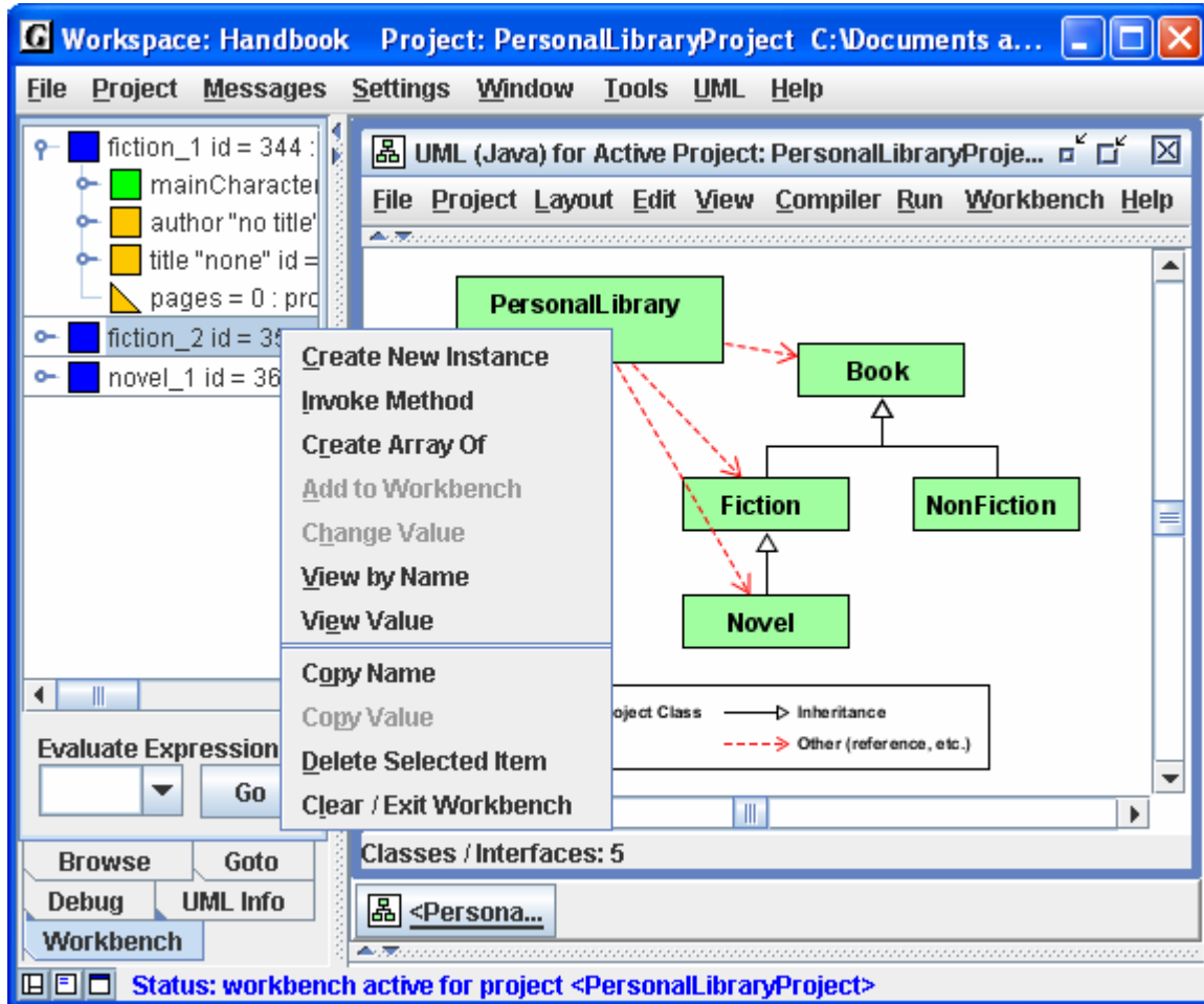
Figure 6-8. Workbench with two instances of Fiction
