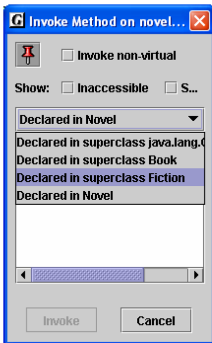
Figure 6-13. Viewing superclasses for novel_1
