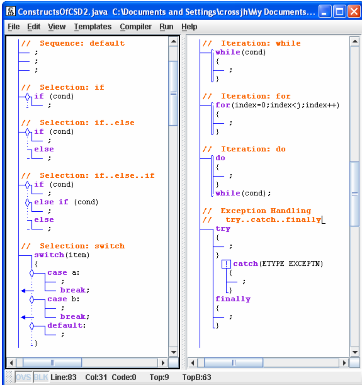
Figure 8-3. CSD Control Constructs generated in CSD Window
