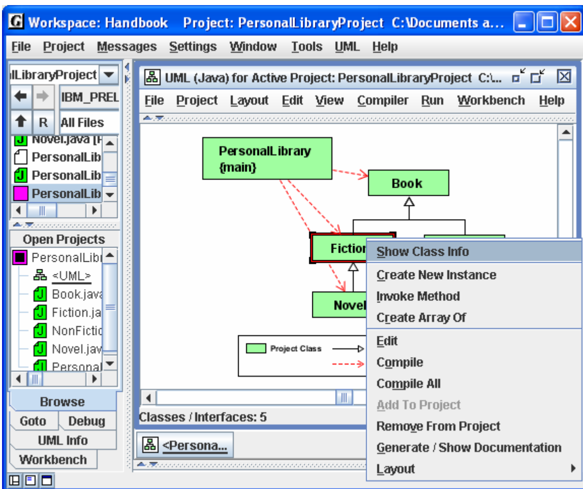
Figure 6-5. Creating an Object for the Workbench
