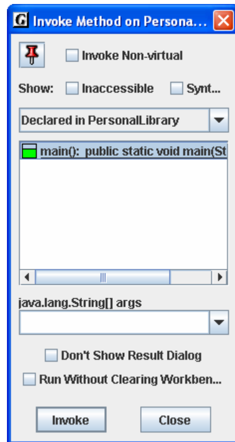
Figure 6-2. Invoking main
